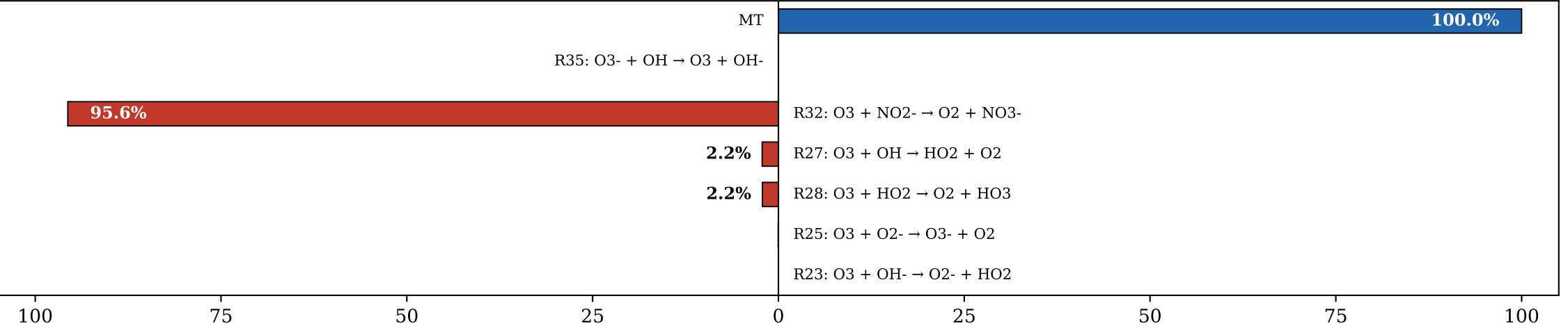
(c) NO 2 - (Σsrc = 2.15e-07 M/s)
